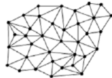
Blockchain Register
