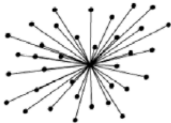
Traditionelles Register
