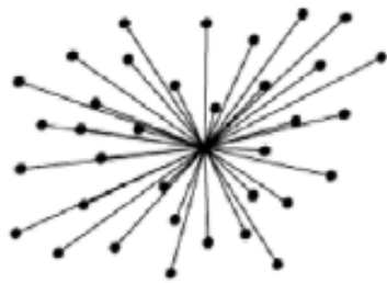
Traditionelles Register
